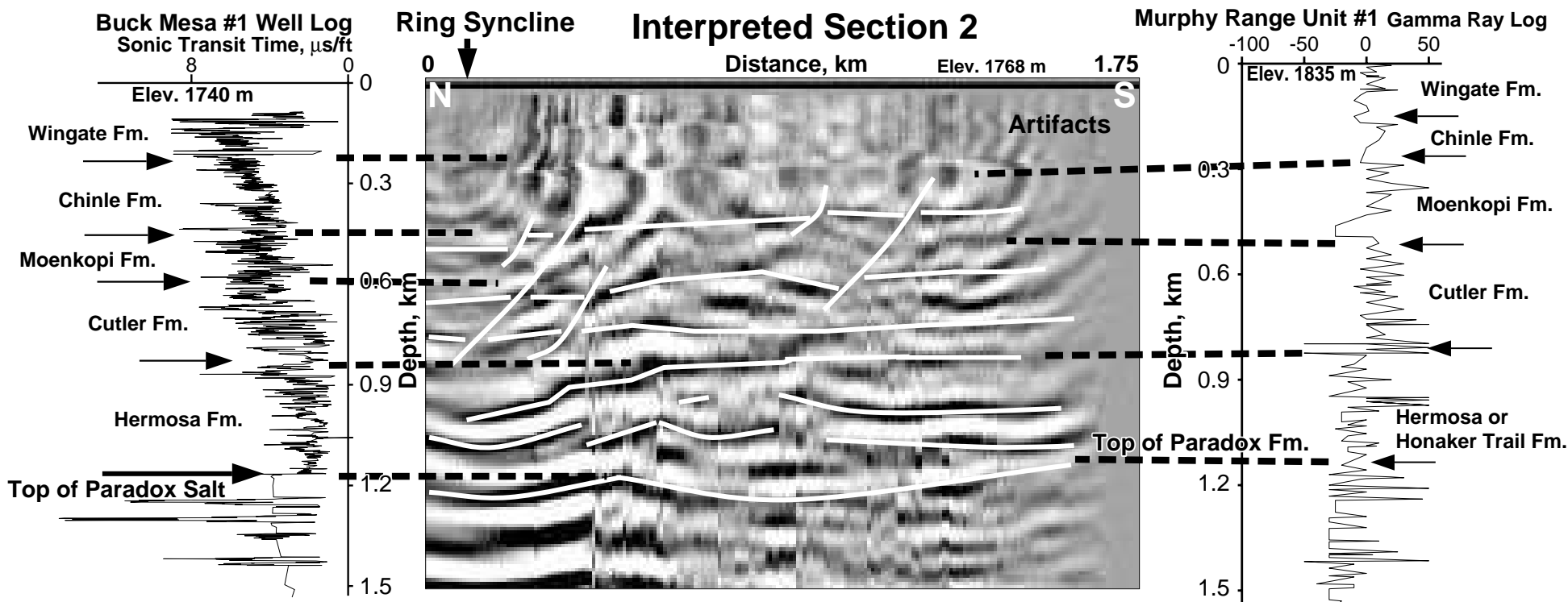
Interpretation of Section 2 (radial to Dome), with log correlations to the top of the Paradox by Herkenhoff (for Buck Mesa well) and Superior Oil (for Murphy Range well). White lines show interpreted faults as well as stratigraphy. Note the 90 m thinning of the Cutler, Moenkopi, and Chinle Formations at the Buck Mesa well in the Ring Syncline, as compared to their thicknesses at the Murphy Range well, outside the zone of deformation. While the seismic section does suggest deformation of the Hermosa Formation, there is no comparable deflection of the top of the Paradox salt.
