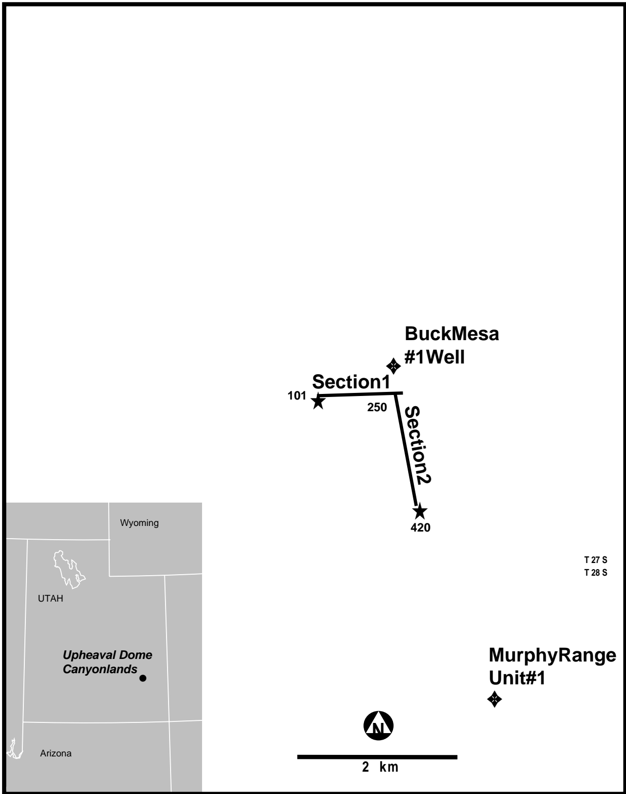
Map showing the location of the reflection line and 2 wells at Upheaval Dome, Canyonlands National Park, Utah. Well locations shown are approximate. Seismic sections 1 and 2 are located between station numbers 101 and 250, and 250 and 420 respectively. Geologic map from Huntoon et al. (1982).
