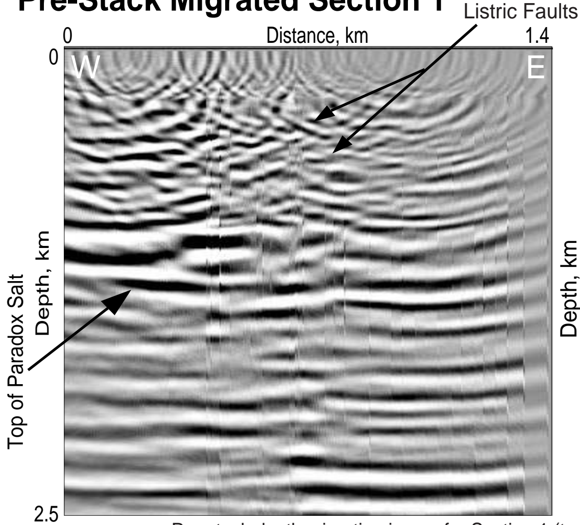
Pre-stack depth migration image for Section 1 (transverse direction), with Buck Mesa #1 well sonic log. The top and bottom of the Paradox salt correlate well with the log, despite migration artifact arcs. Images of listric faults appear above the salt.
