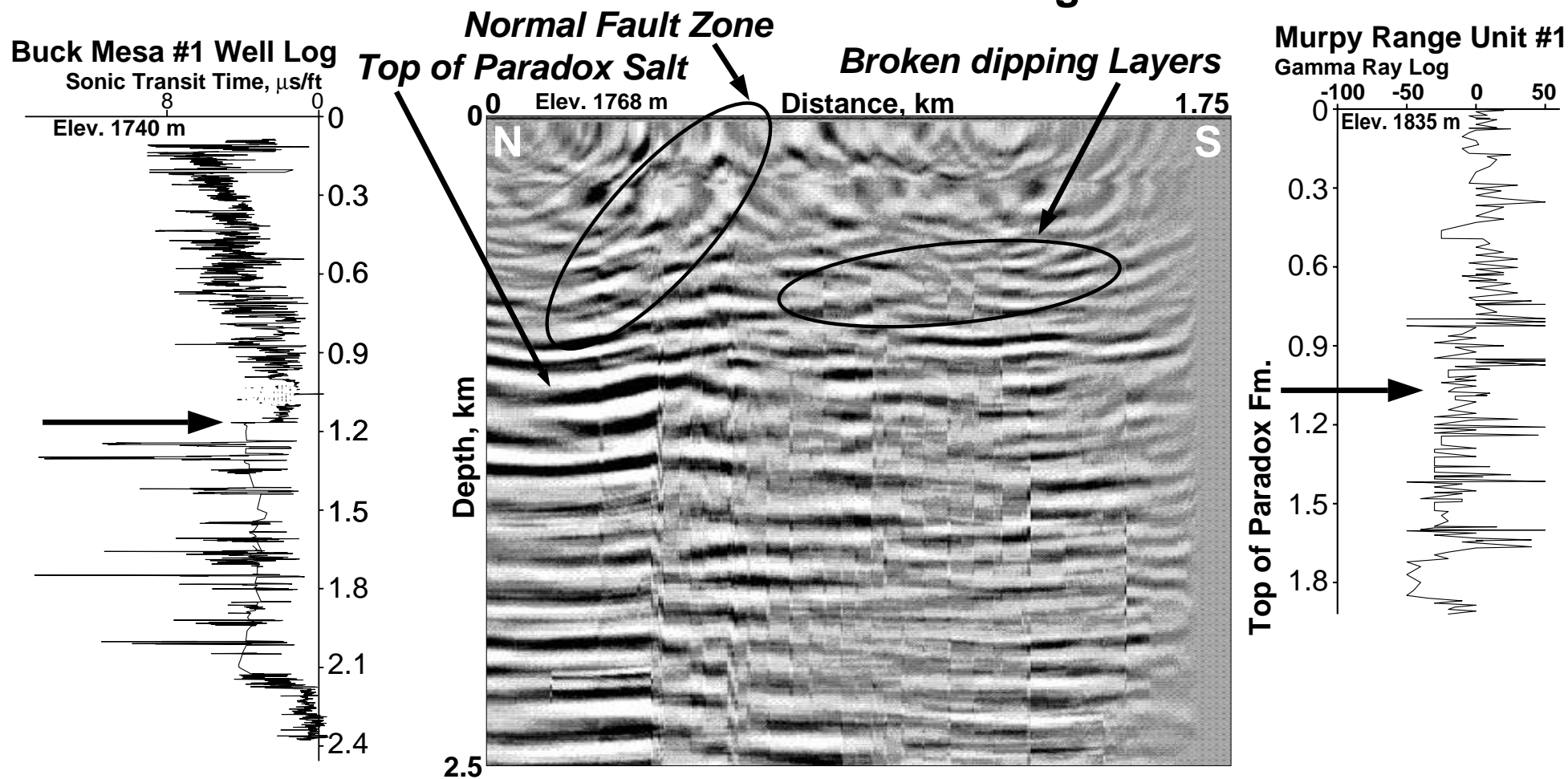
Pre-stack depth migration image for Section 2 (radial direction), with Buck Mesa #1 well sonic log and Murphy Range Unit #1 gamma ray log. The top of the Paradox salt correlates well with the logs, despite migration artifact arcs. Images of normal fault planes and fault-broken stratigraphy appear above the salt.
