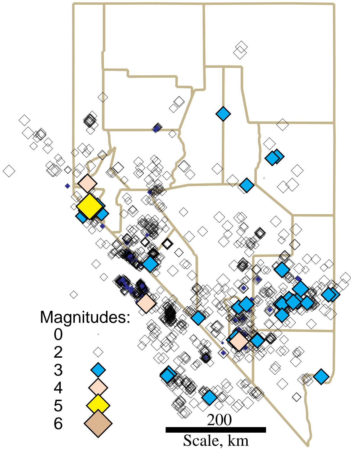
Fig. 1: 2907 events recorded during the calendar year 1994 in Nevada and eastern California by the University of Nevada, Reno Seismological Laboratory.
