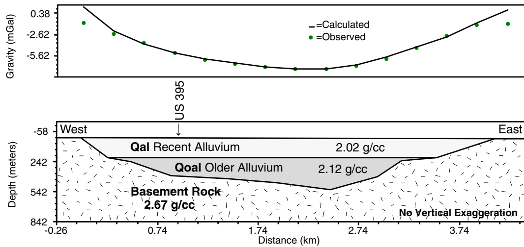
FIGURE. 2.13. Carson City-Eagle Valley 5th street gravity cross section (location given in Figure 2.11) computed by 2.5-D forward modeling. Layering in basin sediments follow scheme in Table 2.2. No vertical exaggeration.
