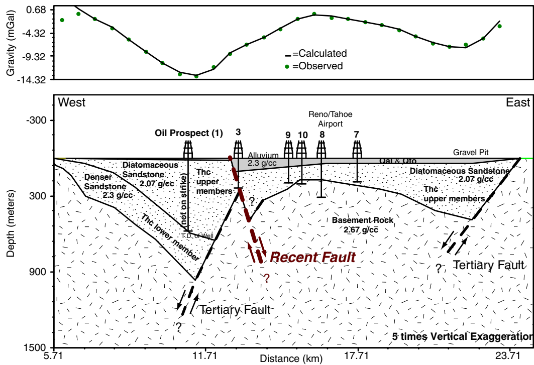
FIGURE 2.8. Reno-Truckee Meadows Truckee River gravity (location given in Figure 2.7) cross-section as computed by 2.5-D forward modeling. Wells with numbers refer to Figure 2.7 and Table 2.1. Vertical exaggeration is 5 times.
