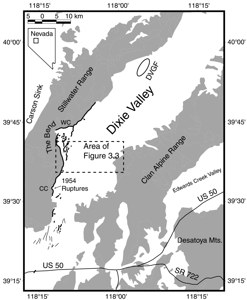
FIGURE 3.1. Map of Dixie Valley, Nevada, and surrounding areas. Shaded areas are mountainous, open areas are basins. Dashed box is area of Figure 3.3. WC, Wood Canyon; CC, Coyote Canyon; DVGf, Dixie Valley geothermal field.
