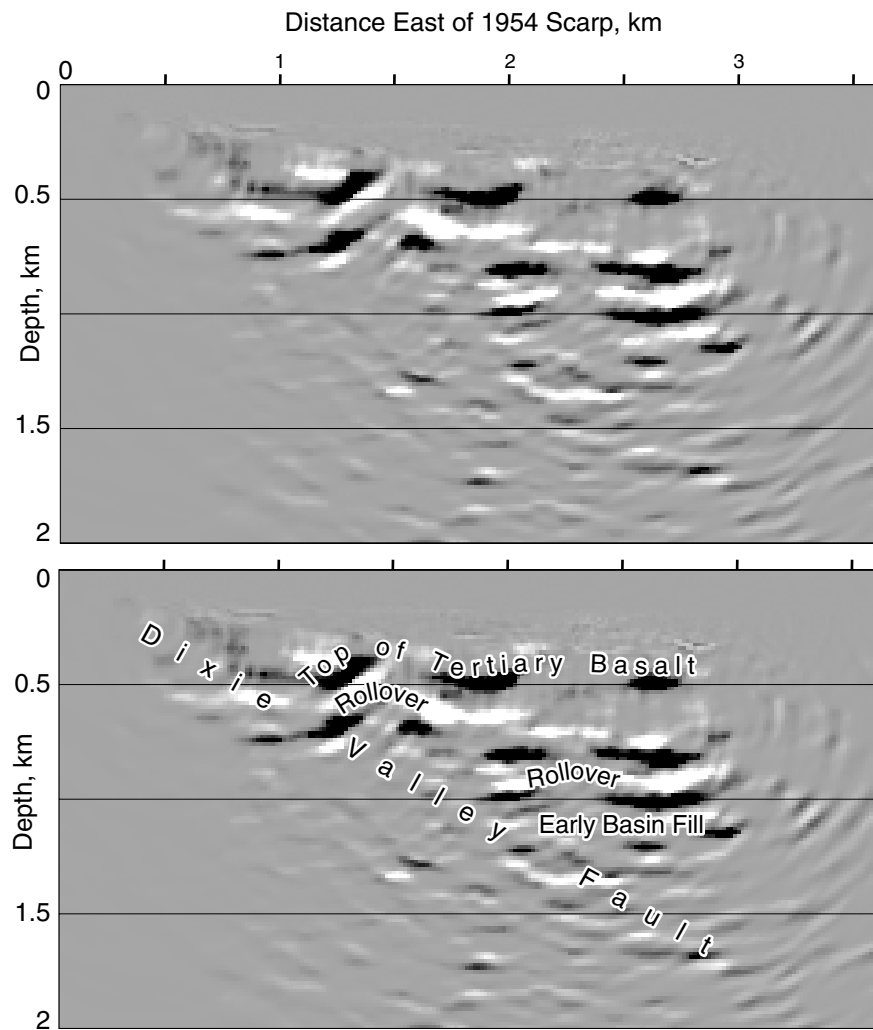
FIGURE 3.8. (top) Kirchhoff prestack migration of our medium-resolution seismic reflection profile. (bottom) Interpreted section. See text for description.
