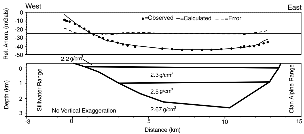
FIGURE 3.9. A 2.5-D gravity model of Dixie Valley at Cattle Road (Figure 3.3). Circles are observed gravity, and dashed line is model misfit. Fault dips to east at \sim 26^\circ .
