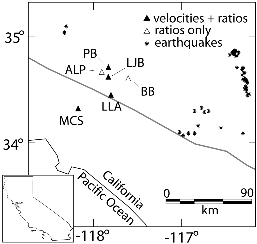
FIGURE 4.1. Basemap showing our site locations. LJB is Lovejoy Buttes; PB is Piute Butte; ALP is Alpine Butte; BB is near Black Butte; MCS is Mill Creek Summit; and LLA is Llano.
