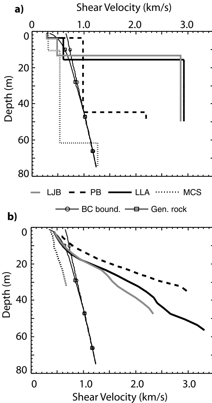
FIGURE 4.3. Shear-velocity models from modeling of refraction-microtremor dispersion curves (a), and laterally averaging P-wave tomography results assuming 0.25 Poisson's ratio (b). NEHRP BC boundary [Frankel et al., 1996] and "generic rock" [Boore and Joyner, 1997] profiles are plotted for reference.
