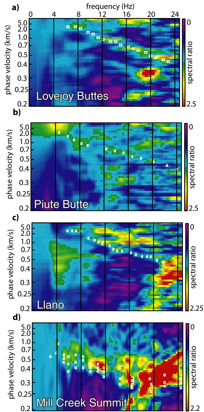
FIGURE 4.4. Velocity-frequency plots from data recorded at our sites. Warmer colors indicate more seismic energy at that velocity-frequency coordinate. White boxes are dispersion curve picks we used to model shear-wave velocity. See Louie [2001] for details on the method.
