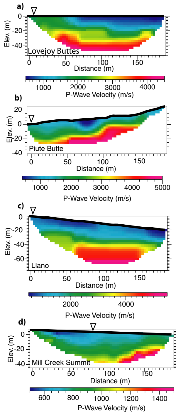
FIGURE 4.5. P-wave velocity models obtained by optimization of refracted first-arrivals. Triangles are located at the approximate location of the 3-component measuring station.
