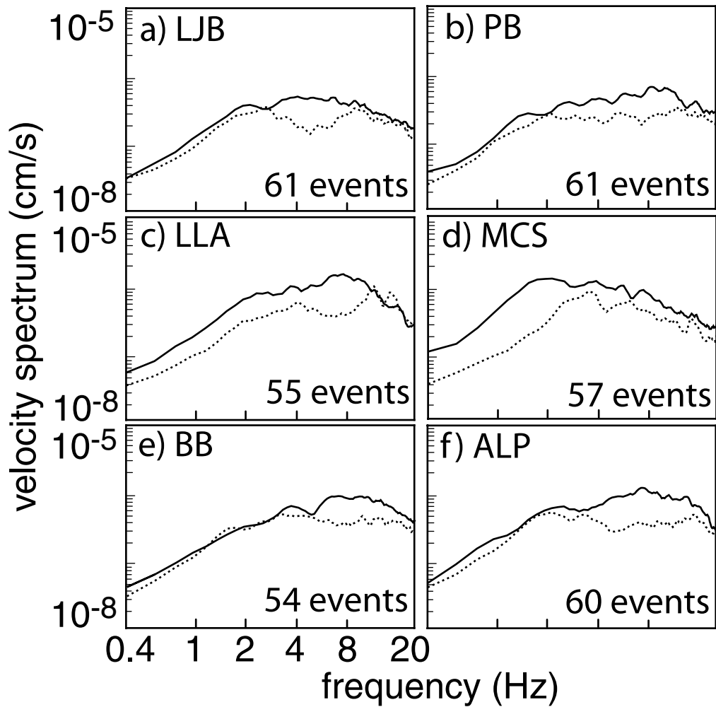
FIGURE 4.6. Horizontal (solid) and vertical (dashed) velocity amplitude spectra. The spectra are the result of logarithmically summing the smoothed spectra of the number of events indicated.
