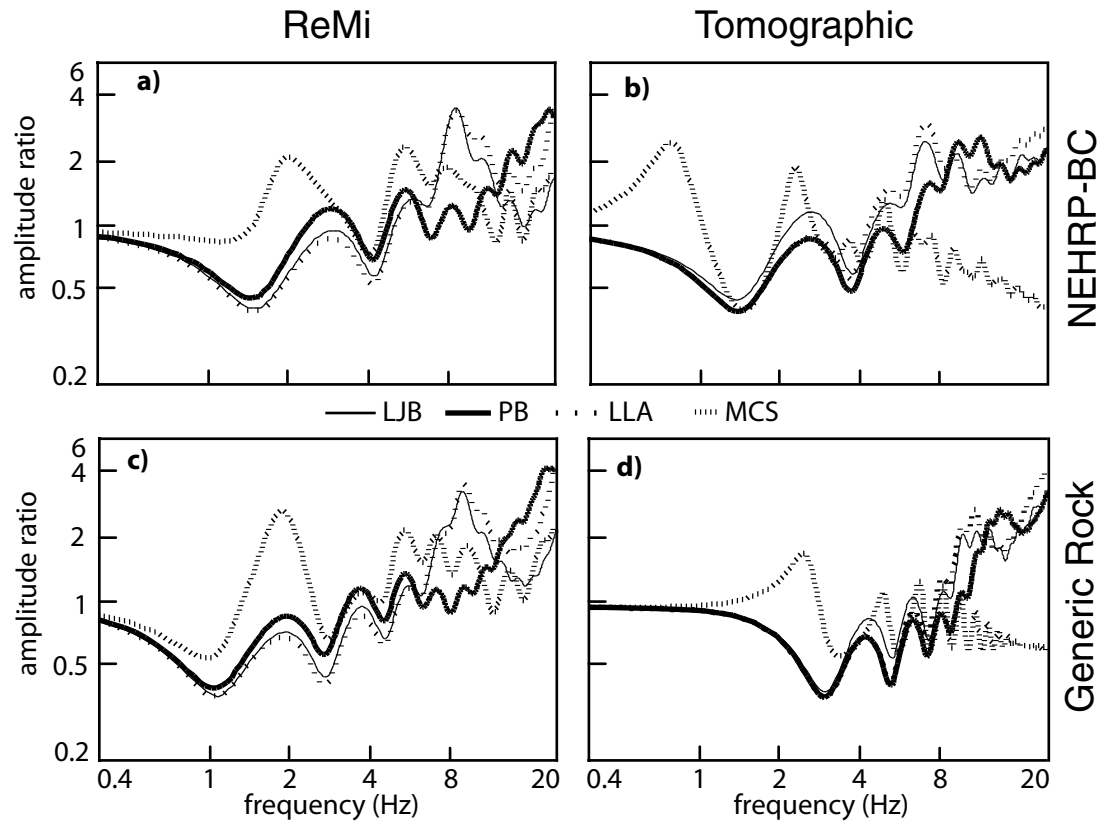
FIGURE 4.8. Synthetic spectral ratios relative to NEHRP BC boundary [Frankel et al., 1996] from ReMi velocities (a) and tomography velocities (b), and synthetic spectral ratios relative to "generic rock" [Boore and Joyner, 1997] from ReMi velocities (c) and tomography velocities (d).
