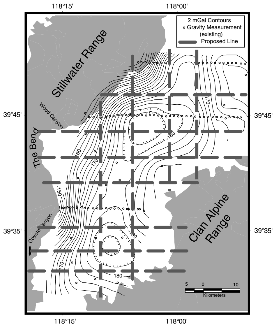
FIGURE 5.2. Gravity map of Dixie Valley with proposed transects. 2 mGal contours and existing gravity points are from Schaefer [1982]. Gravity coverage extends to all areas of the map (and beyond), but only basin contours are shown. Basin gravity lows are correlated with possible low-angle fault to high-angle fault accommodation zones. Proposed gravity transects are dashed lines.
