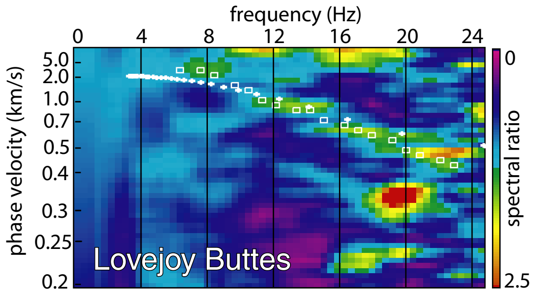
FIGURE 5.3. Comparison dispersion curves from tomography velocity model (crosses) and ReMi picks.
