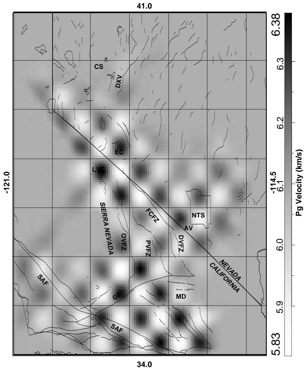
Figure 2.11: Output P_g velocity model obtained from a checkerboard sinusoidal test model with cell sizes of 0.5^\circ by 0.5^\circ .
