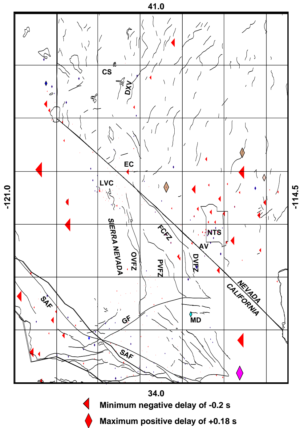
Figure 2.12: Output station delays obtained from a checkerboard sinusoidal test model with cell sizes of 0.5^\circ by 0.5^\circ . Only stations with non-zero error are shown.
