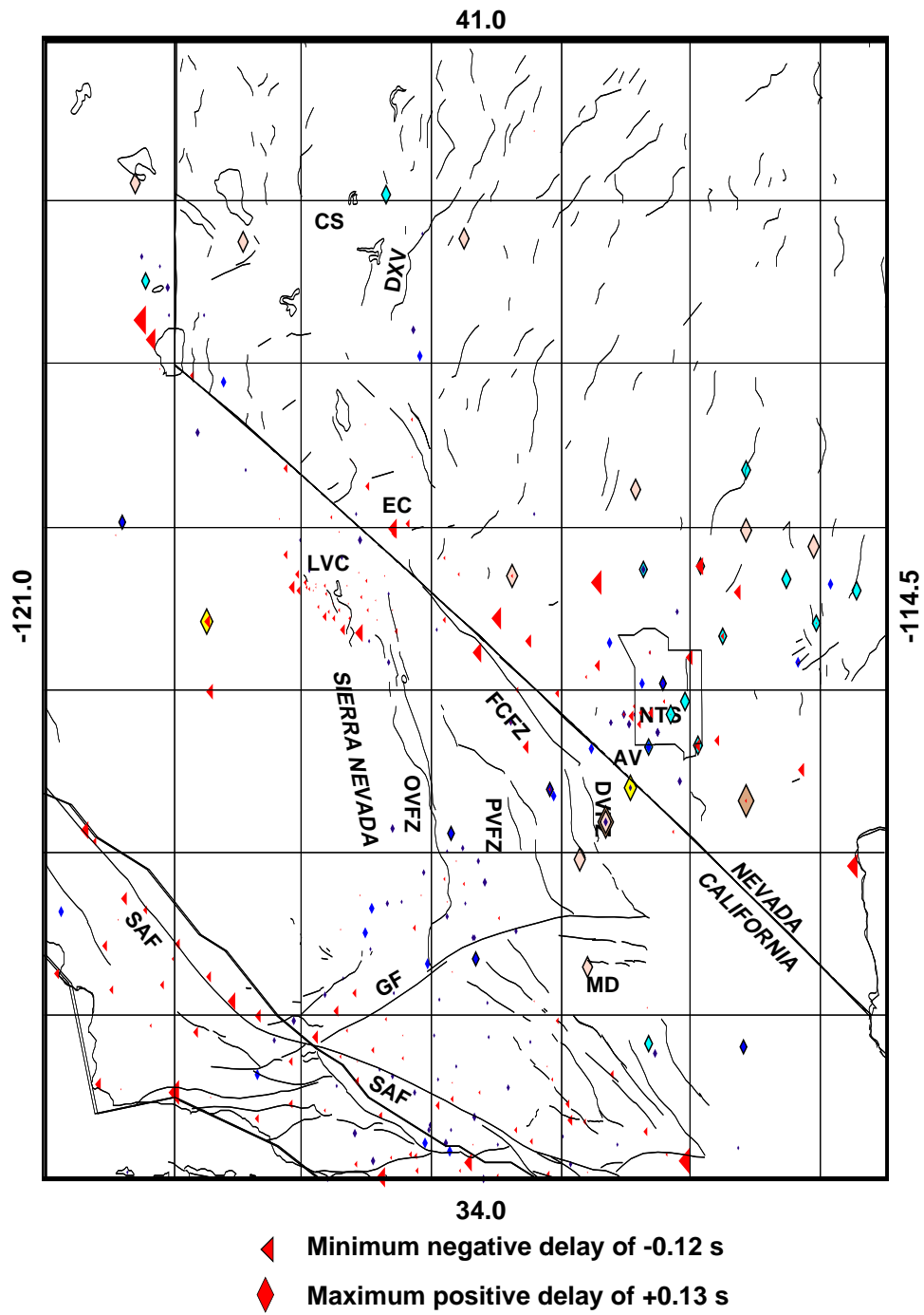
Figure 2.14: Output station delays obtained from a checkerboard sinusoidal test model with cell sizes of 0.25^\circ by 0.25^\circ . Only stations with non-zero error are shown.
