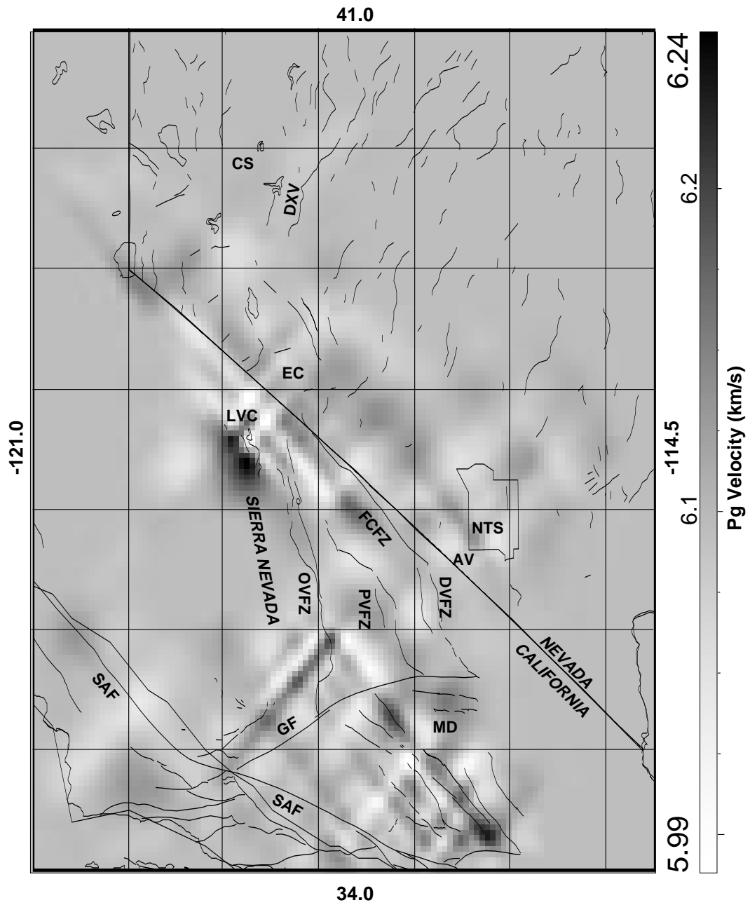
Figure 2.15: Output P_g velocity model obtained from a checkerboard sinusoidal test model with cell sizes of 0.17^\circ by 0.17^\circ .
