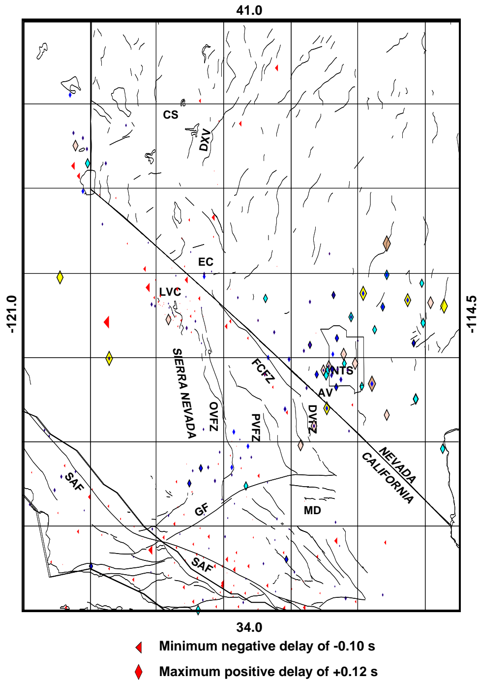
Figure 2.16: Output station delays obtained from a checkerboard sinusoidal test model with cell sizes of 0.17^\circ by 0.17^\circ . Only stations with non-zero error are shown.
