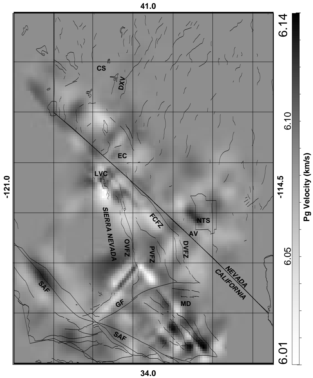
Figure 2.17: Output P_g velocity model obtained from a checkerboard sinusoidal test model with cell sizes of 0.10^\circ by 0.10^\circ .
