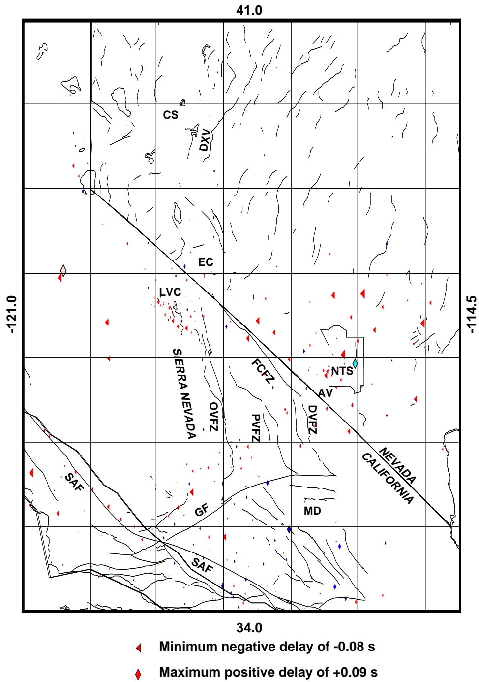
Figure 2.18: Output station delays obtained from a checkerboard sinusoidal test model with cell sizes of 0.10^\circ by 0.10^\circ . Only stations with non-zero error are shown.
