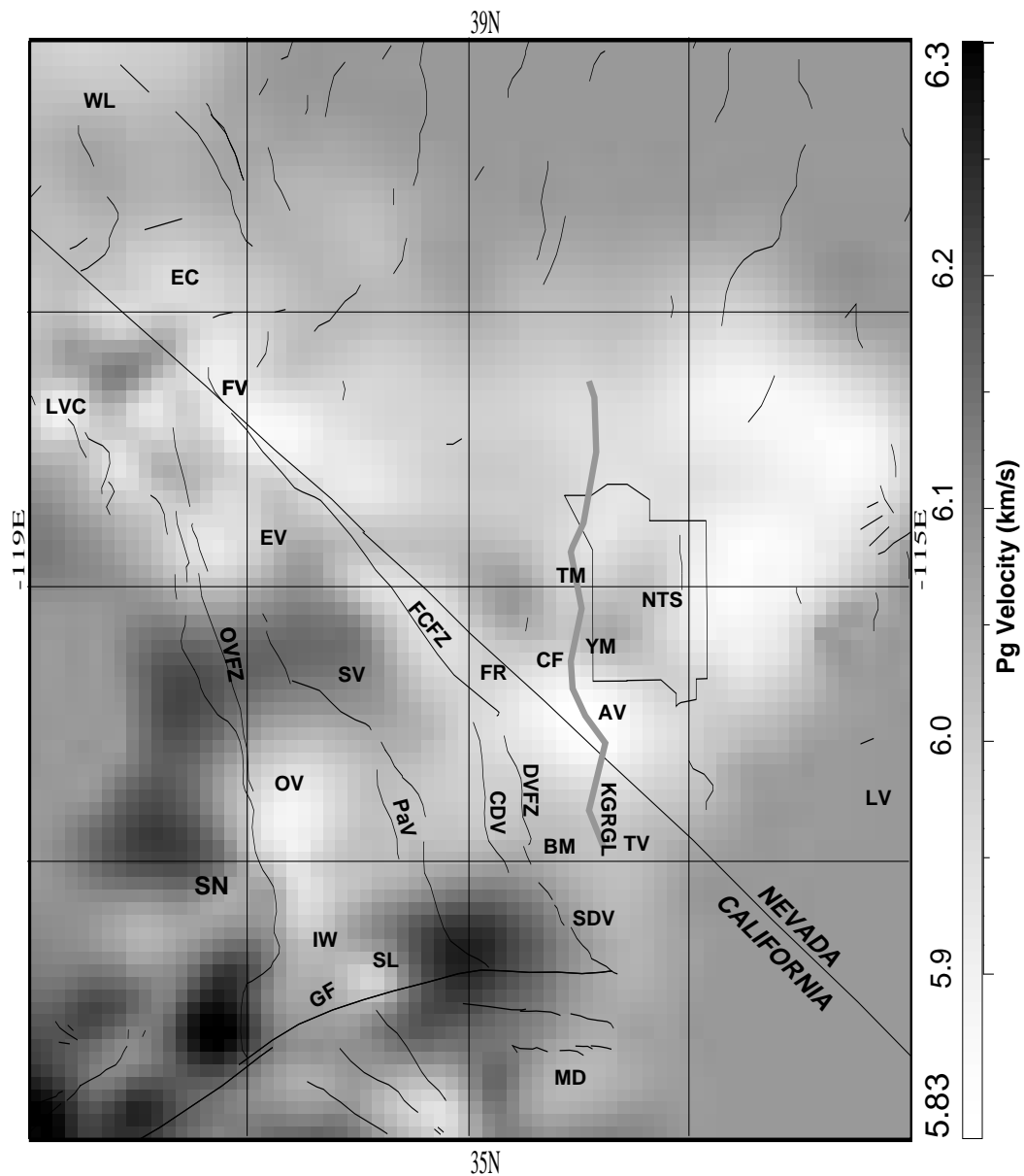
Figure 2.19: Expanded display of the central part of Figure 2.6. Abbreviations: AV=Amargosa Valley, BM=Black Mountains, CDV=Central Death Valley, CF=Crater Flat, DVFZ=Death Valley Fault Zone, EC=Excelsior-Coaldale, EV=Eureka Valley FCFZ=Furnace Creek fault zone, FR=Funeral Range core complex, FV=Fish Lake Valley, GF=Garlock Fault, IW=Indian Wells, KGRGL=Kawich-Greenwater Rift gravity low, LV=Las Vegas, LVC=Long Valley Caldera, MD=Mojave Desert, ML=Mono Lake, NDV=northern Death Valley, NTS=Nevada Test Site, OV=Owens Valley, OVFZ=Owens Valley Fault Zone, PaV=Panamint Valley, SAF=San Andreas Fault, SDV=Southern Death Valley, SL=Searles Lake, SN=Sierra Nevada, SV=Saline Valley, TM=Timber Mountain caldera complex, TV=Tecopa Valley, WL=Walker Lake, YM=Yucca Mountain
