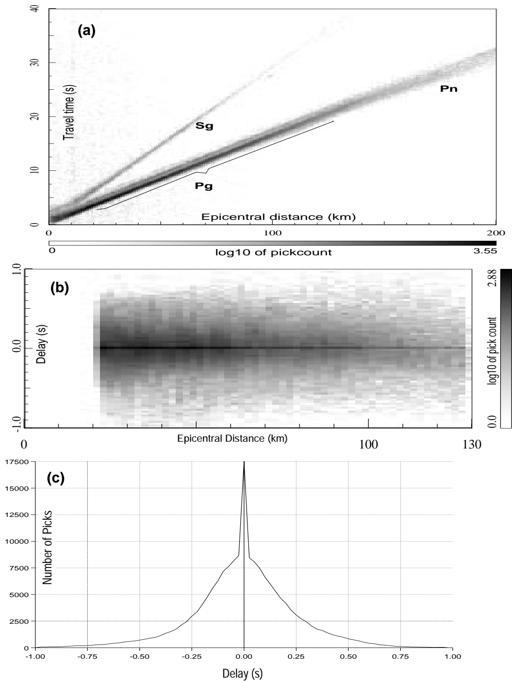
Figure 2.3: a) Gray scale plot of travel time versus epicentral distance for the input data set. Darkness increases with hit count. b) Gray scale plot of delay times with respect to the average best-fitting velocity. c) Histogram of delays.
