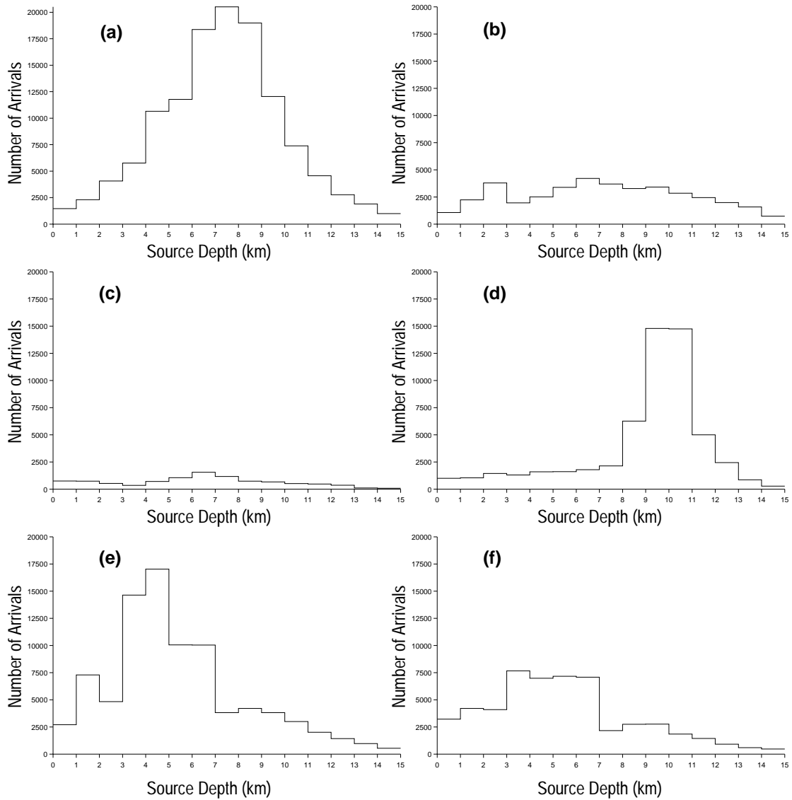
Figure 2.4: Histogram of earthquake source depths for P_g wave arrivals in six different subregions. a) Long Valley Caldera-Mammoth Lakes. b) Northern Nevada. c) Eureka Valley. d) Southern Nevada-Nevada Test Site. e) Owens Valley-Indian Wells. f) Landers (southern Mojave Desert).
