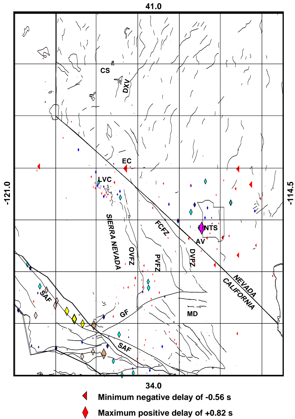
Figure 2.7: Station delays obtained by the tomographic inversion. Abbreviations same as in Figure 2.1. Delays are proportional to the symbol size.
