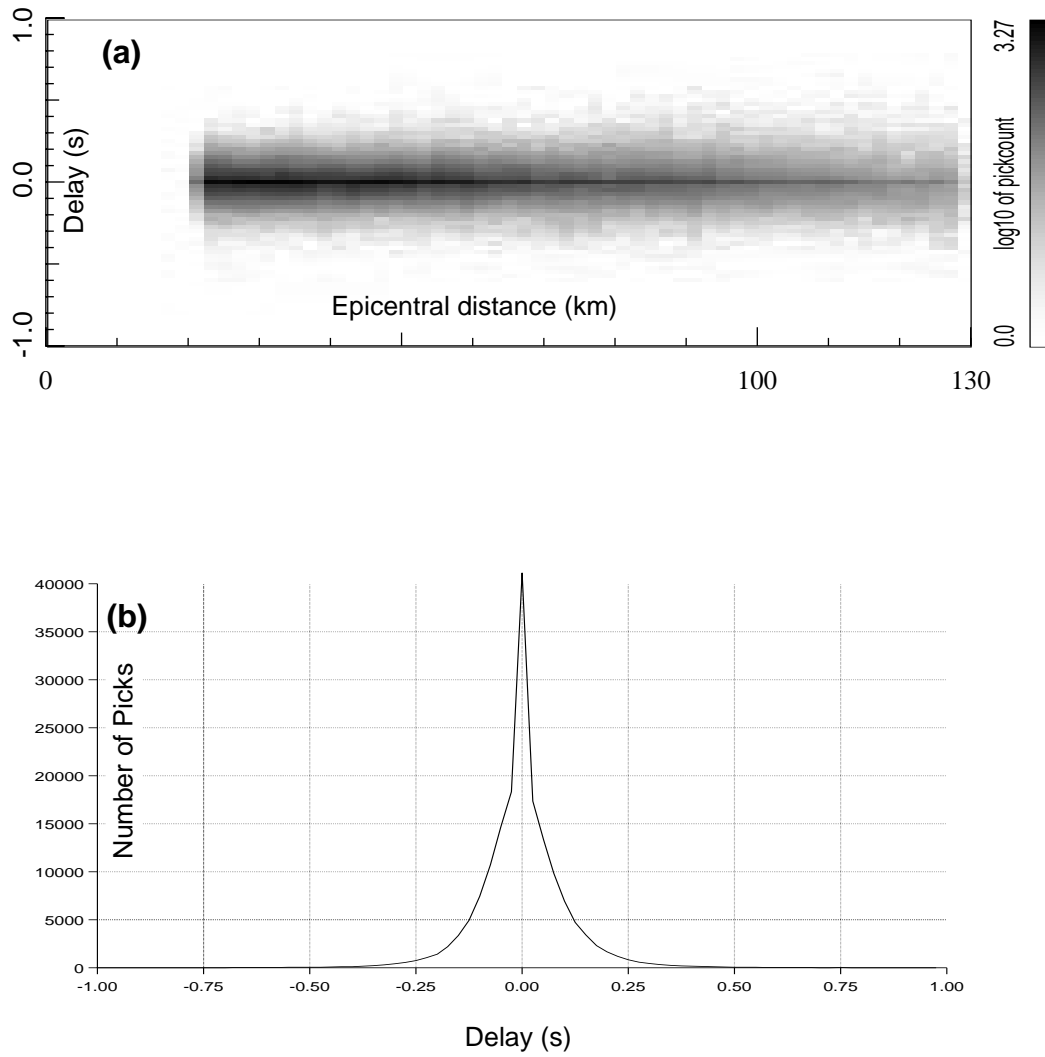
Figure 2.8: a) Gray scale plot of delay times after source and receiver time correction, and projection through the final velocities. b) Corresponding histogram of delays.
