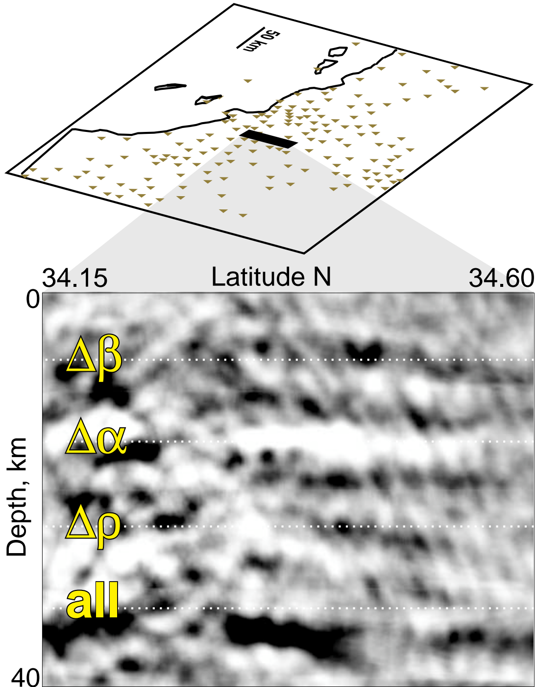
Fig. 3.8. View of the SCSN station locations (above), with depth section from migration of records from five synthetic events (Fig. 3.7) having increasing epicentral depths. The dip-filtered image results from acoustic processing of vertical-component elastic synthetic seismograms (near offset = 15 km; far offset = 175 km). \Delta\beta , \Delta\alpha and \Delta\rho stand for S -wave velocity, P -wave velocity and density interface depths, respectively. Black is reconstructed positive reflectivity, white is reconstructed negative reflectivity, and gray shows little reflectivity.
