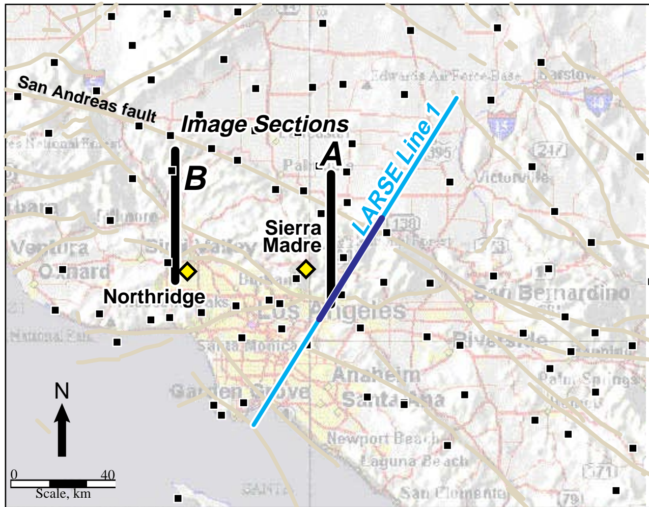
Fig. 4.1. Sierra Madre and Northridge main shocks (diamonds) and aftershock imaging sections (lines A and B) and the LARSE Line 1 section of Fuis et al. (1996; dark on light line) located on topography map of the Los Angeles region. Note the non-parallelism of imaging section A and the LARSE section. Black squares show the locations of some of the network stations I used.
