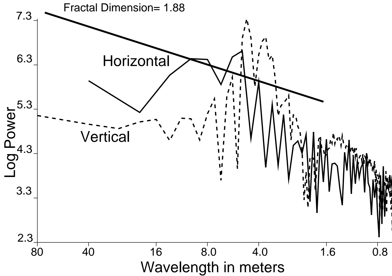
Figure 34 Power spectra for Line D.
