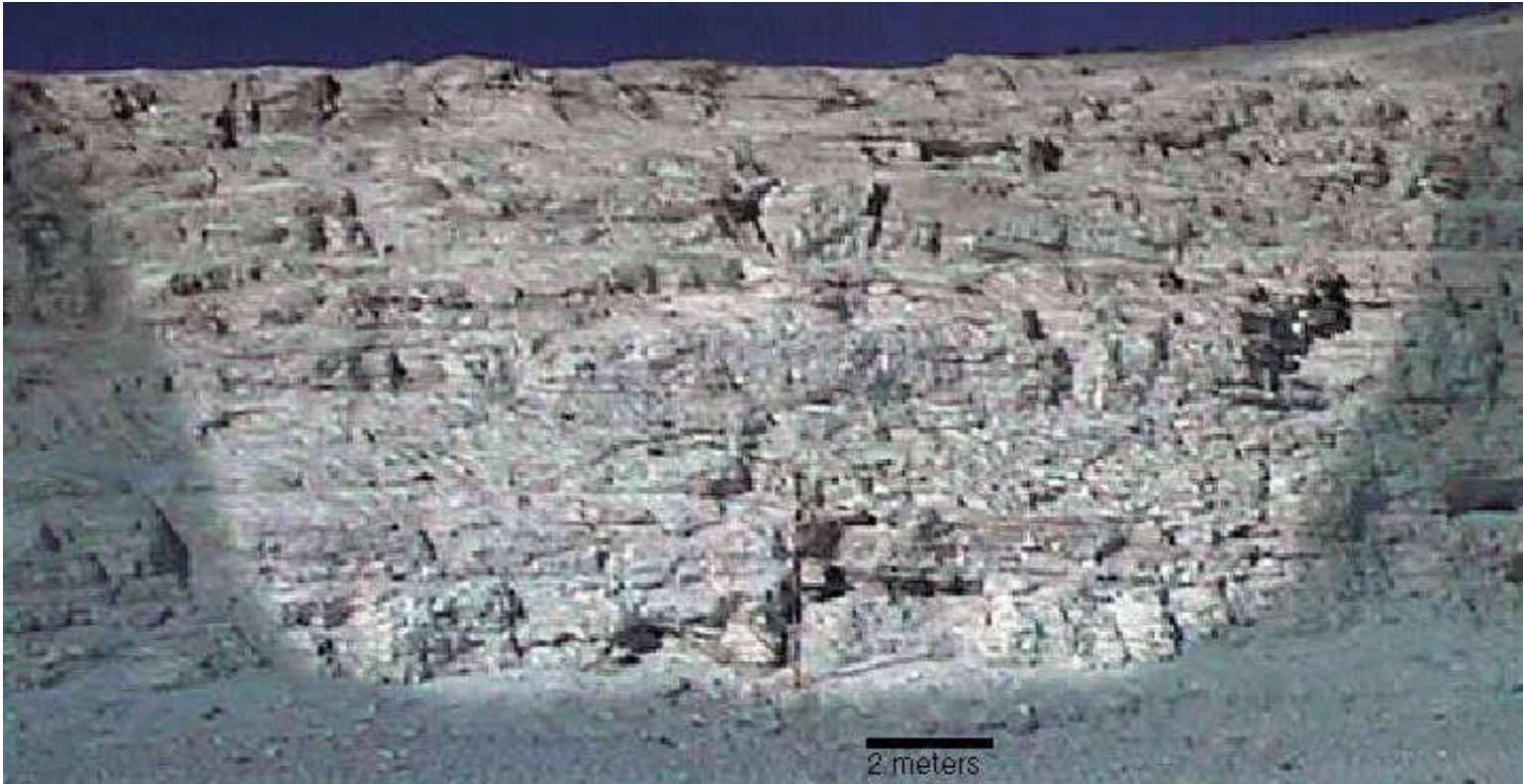
Figure 4 Picture of the face of study from the bottom of the pit with approximate area of full seismic coverage highlighted. The post is 8 feet high. Note the fracture pattern and detail of fracture junctions and compare to the details of the migrated face section (figure 10).
