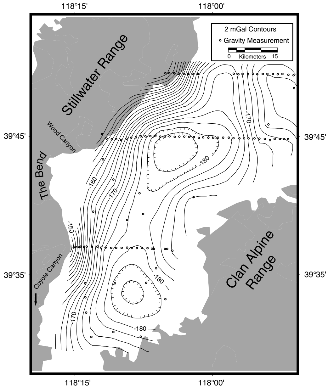
FIGURE 3.2. Complete Bouguer gravity map of Dixie Valley [after Schaefer, 1983]. Gravity contours are at 2-mGal intervals; hachures are on closed minima. Evidence from fault mapping for low-angle Dixie Valley fault dip is between Wood Canyon and Coyote Canyon. Local gravity high between these two latitudes may represent less vertically offset basement rocks.
