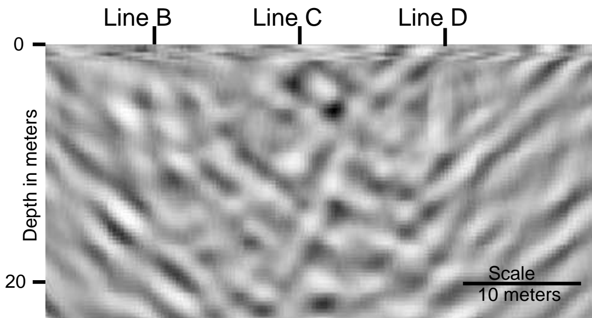
Figure 10 Migrated face line. Note the imaged fracture zone from the middle of the bottom rising to the right and compare to Figure 4.
