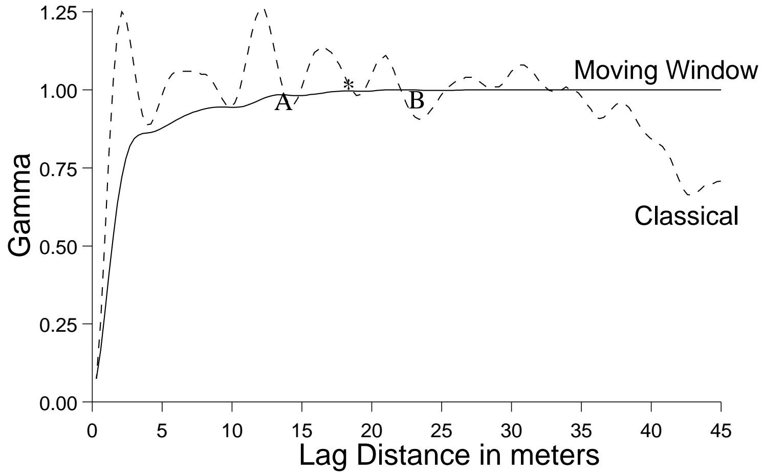
Figure 15 Horizontal variogram for face line
