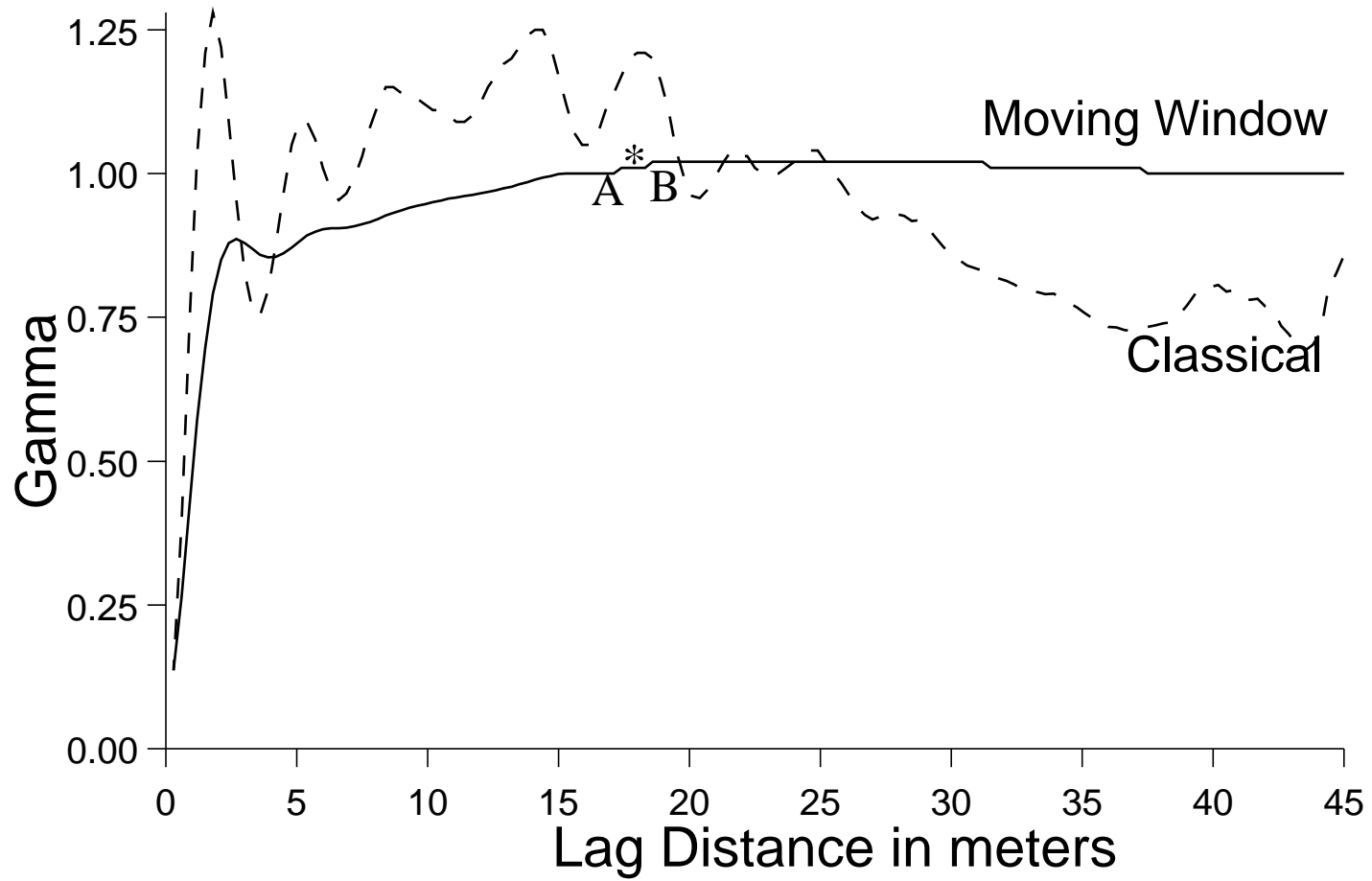
Figure 16 Horizontal variogram for Line A
