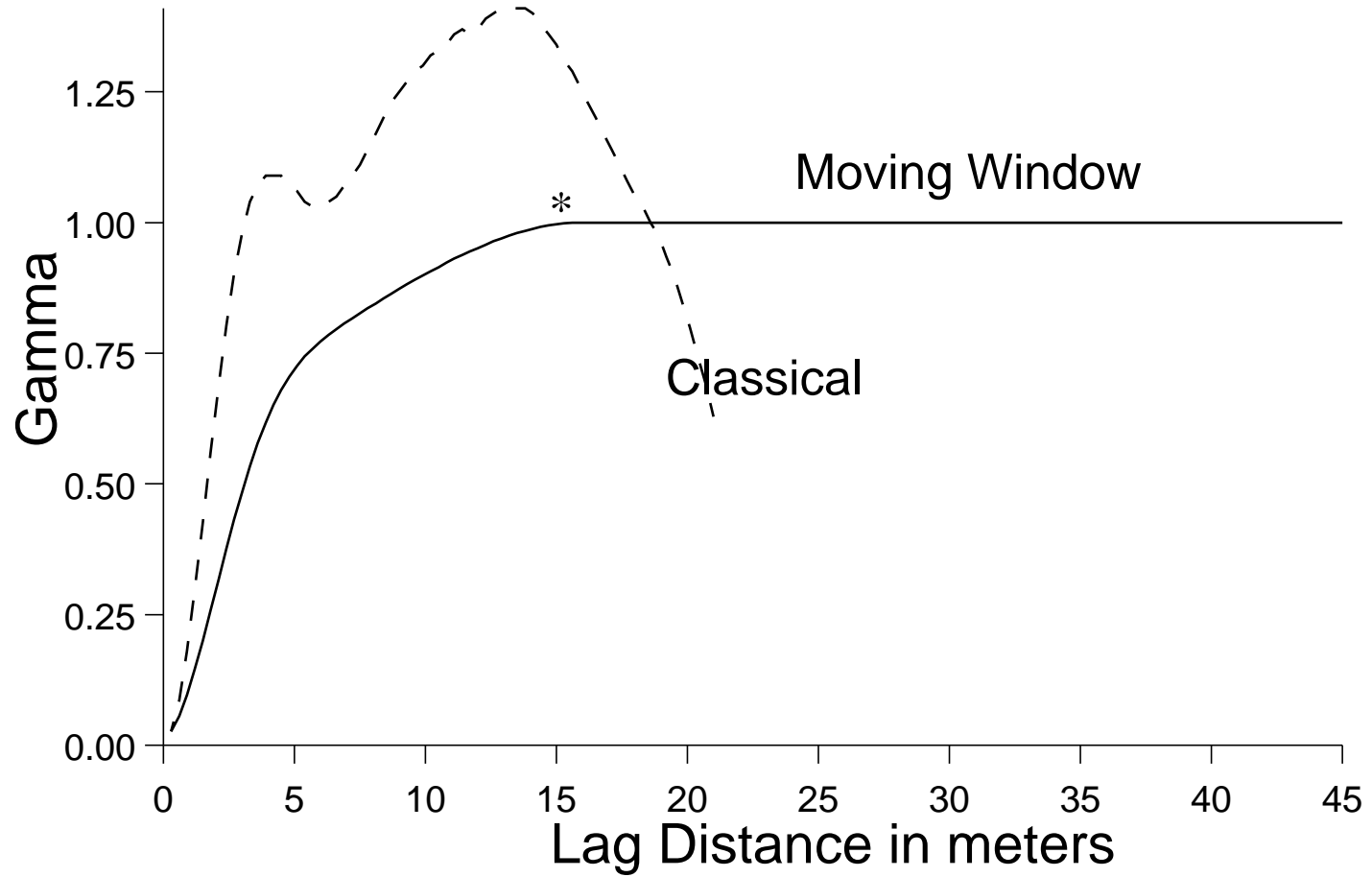
Figure 19 Horizontal variogram for Line D
