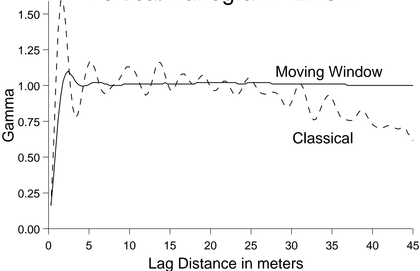
Figure 21 Vertical variogram for Line A
