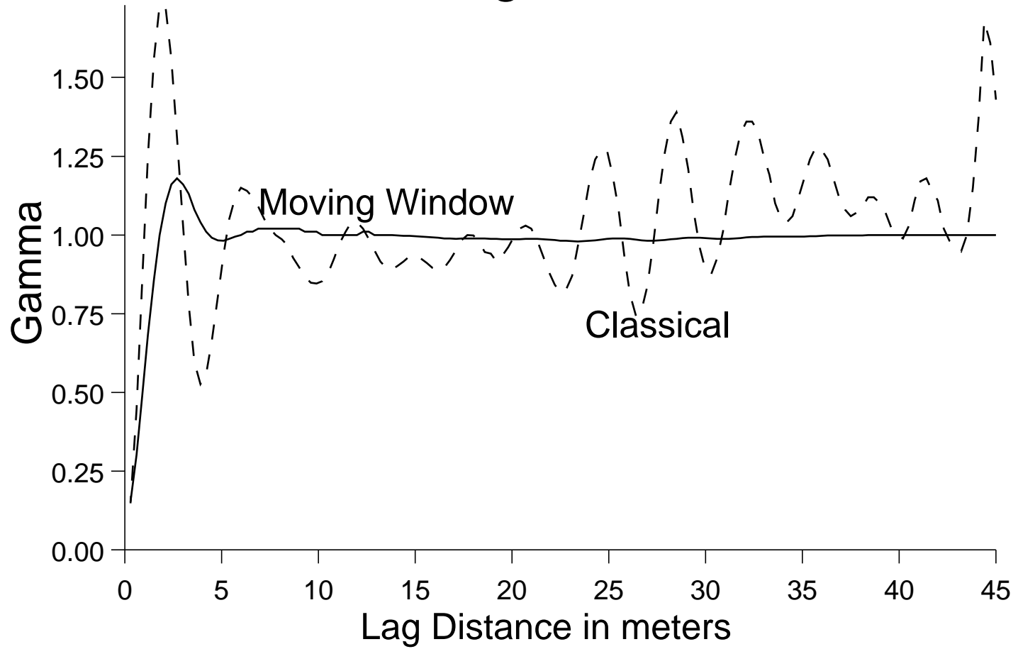
Figure 23 Vertical variogram for Line C
