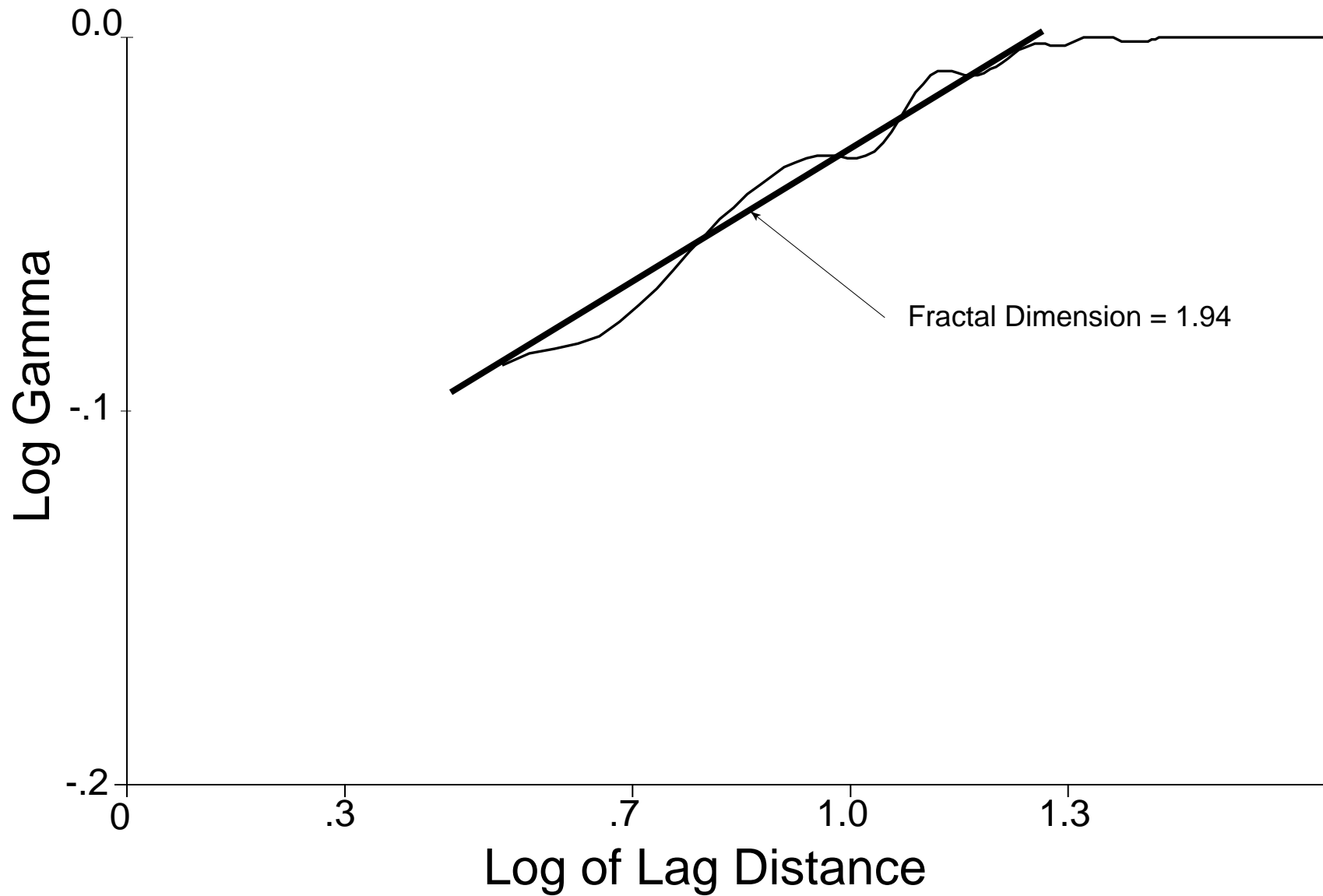
Figure 30 Horizontal variogram for Face Line plotted with a log-log plot
