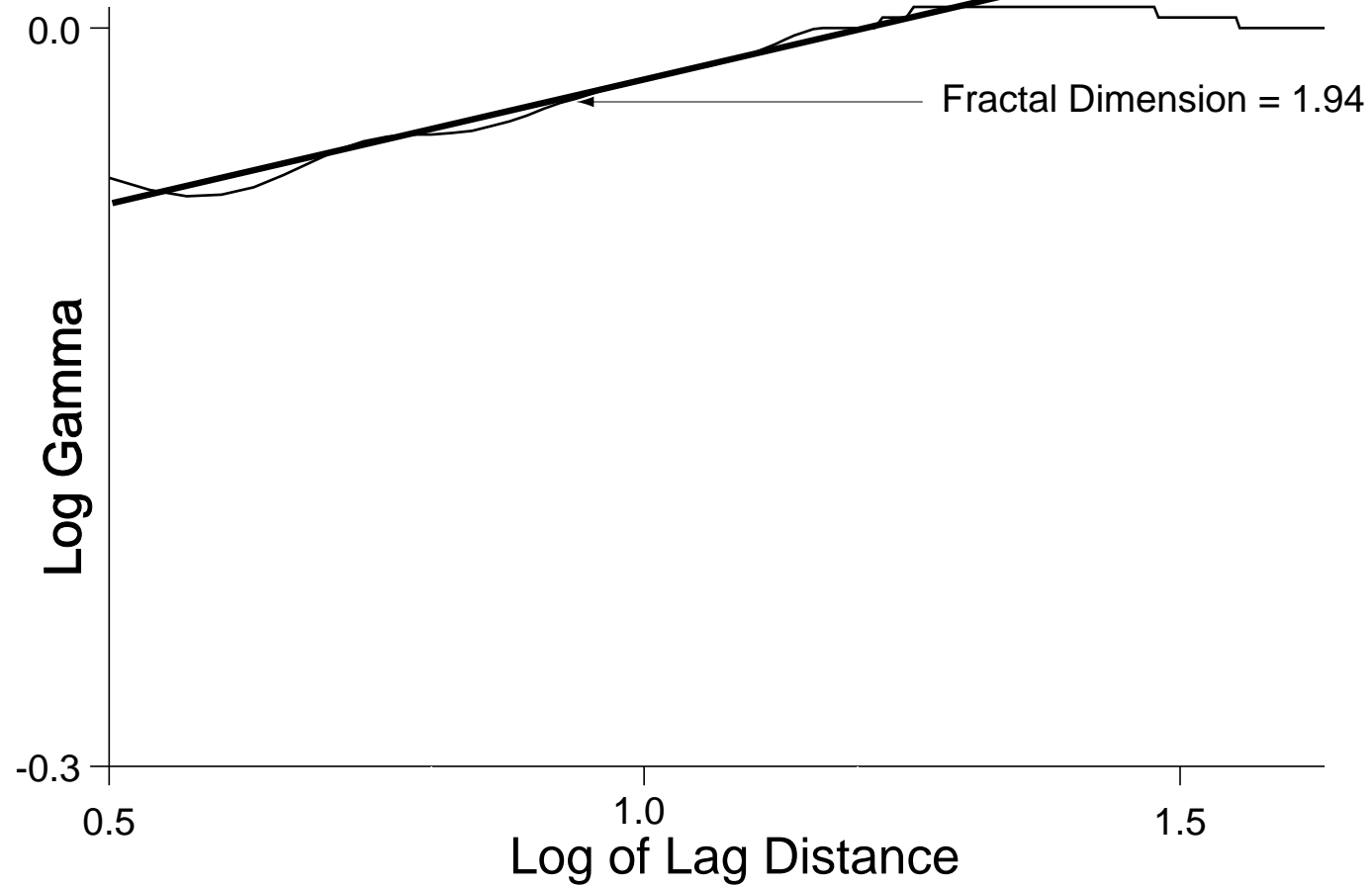
Figure 26 Horizontal variogram for Line A plotted with a log-log plot
