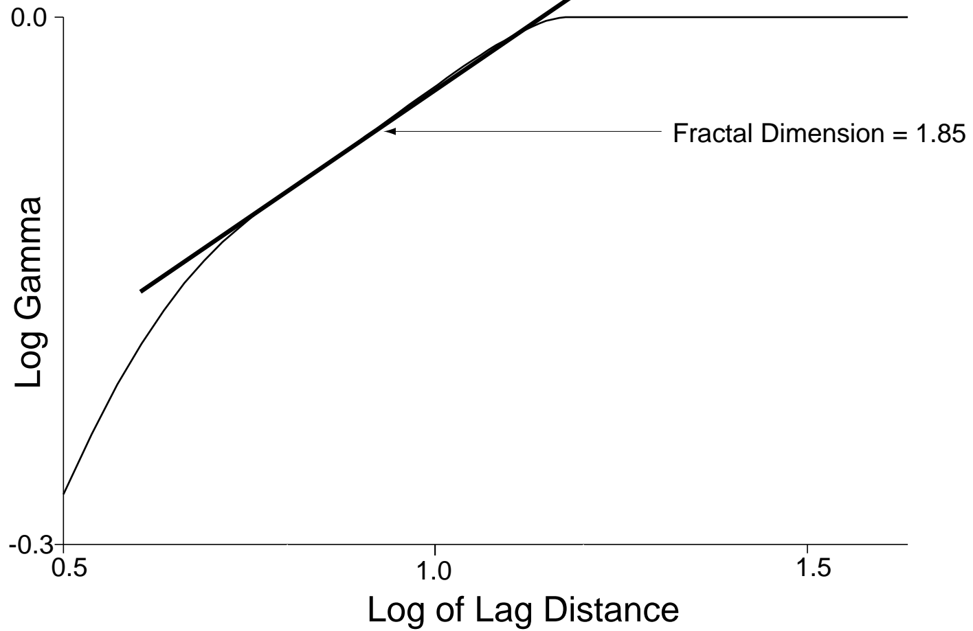
Figure 29 Horizontal variogram for Line D plotted with log-log plot
