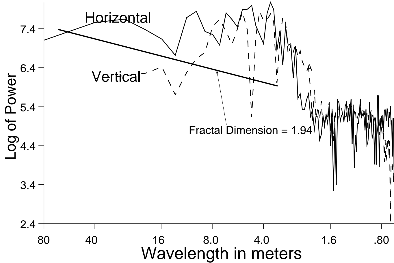
Figure 30 Power spectra for face line.
