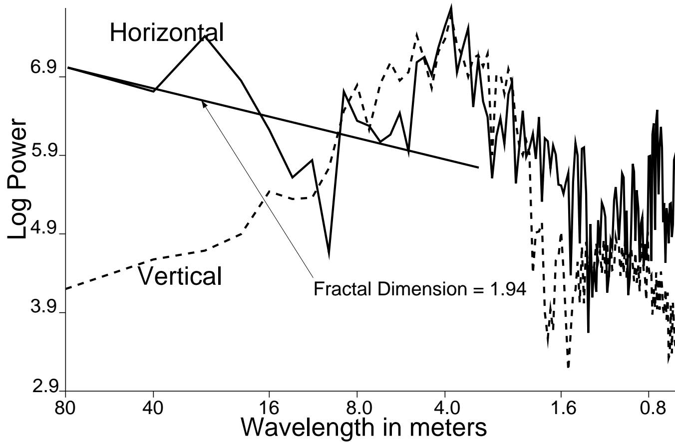
Figure 31 Power spectra for Line A
