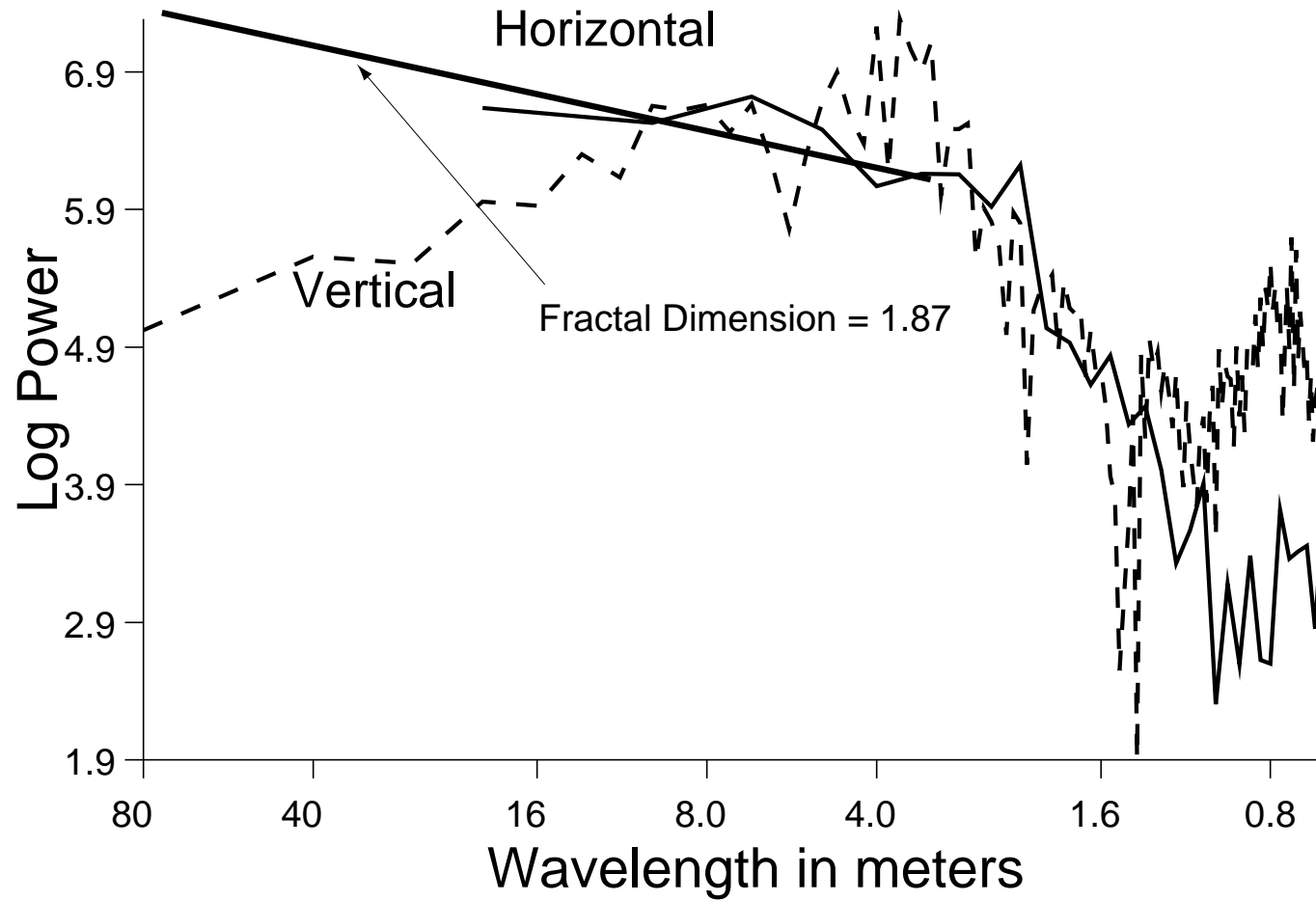
Figure 32 Power spectra for Line B
