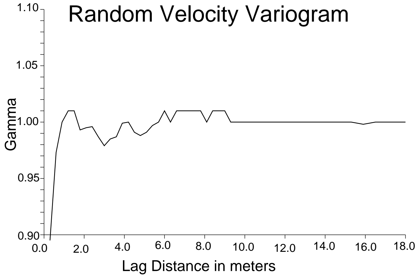
Figure 35 Variogram from random velocity data
