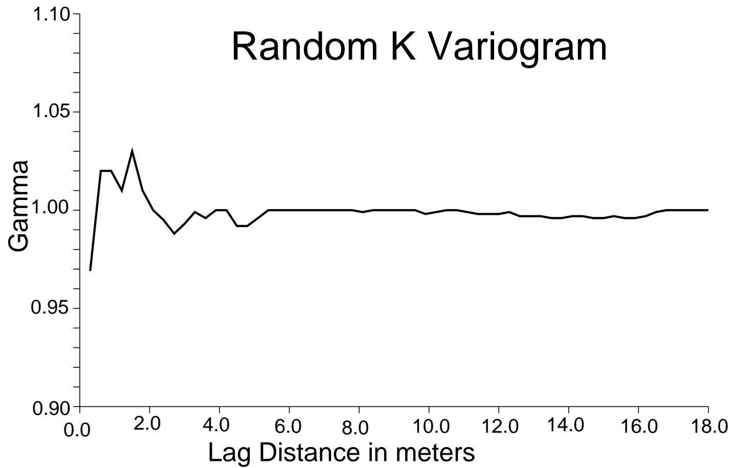
Figure 36 Variogram from hydraulic conductivities calculated from random velocity data.
