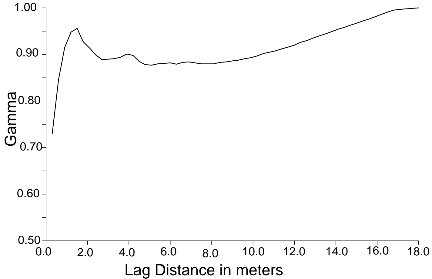
Figure 38 Variogram for hydraulic conductivities calculated from velocity data used for Figure 37
